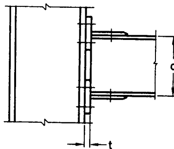
32G T-Stub
