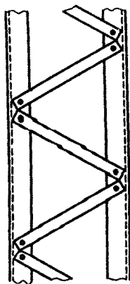
LACING ON FACE A
