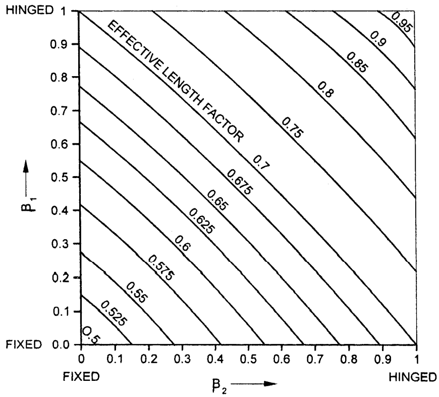
FIG. 27 COLUMN EFFECTIVE LENGTH FACTOR — NON-SWAY FRAME
