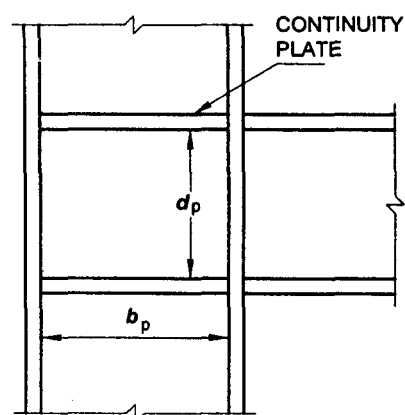
FIG. 21 CONTINUITY PLATES
